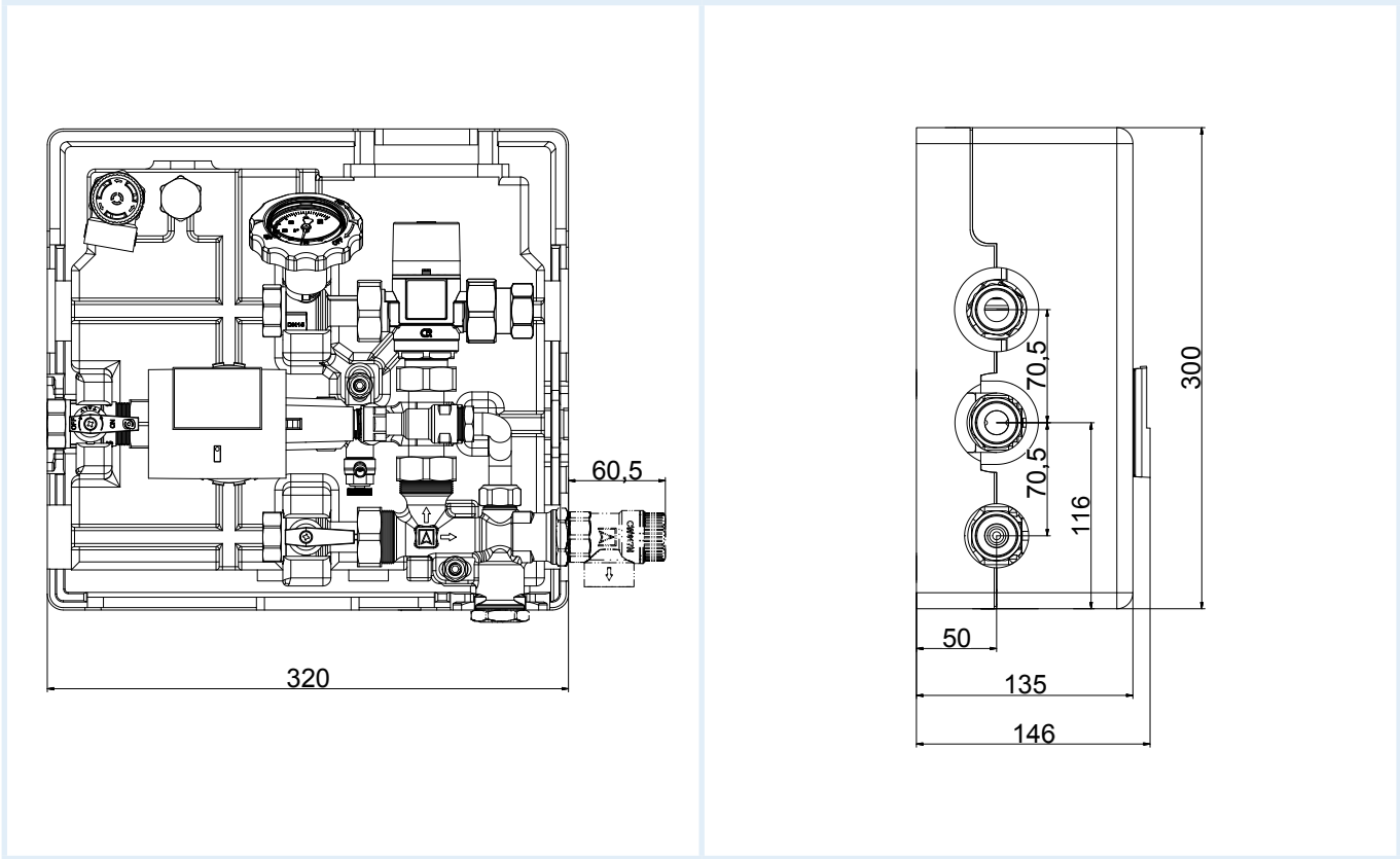
Dimensions (mm)
